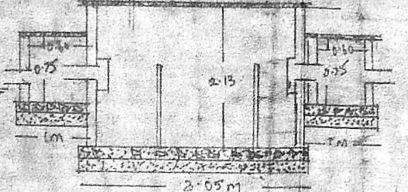
SEPTIC TANK DETAILS SCALE 1CM = 0.54M
